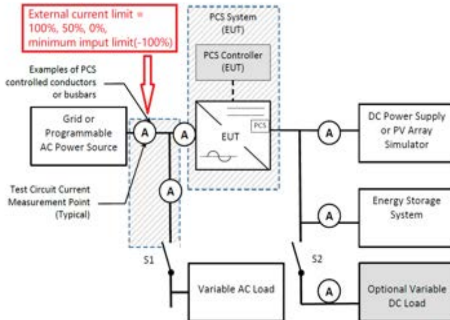
Figure 203.2 – Test Circuit Setup DC Coupled System
