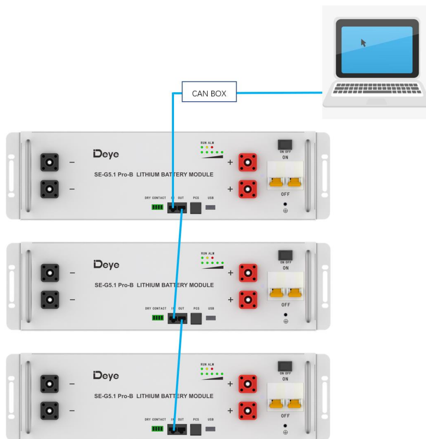
Figure 5-3: Communication Cable Connections between Battery and Computer
