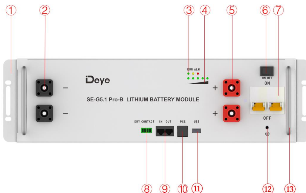
Figure 2-1: Front Panel Function Introduction
