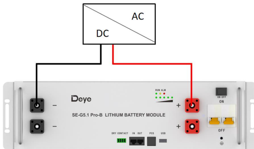
Figure 5-2: Single Battery Connection
