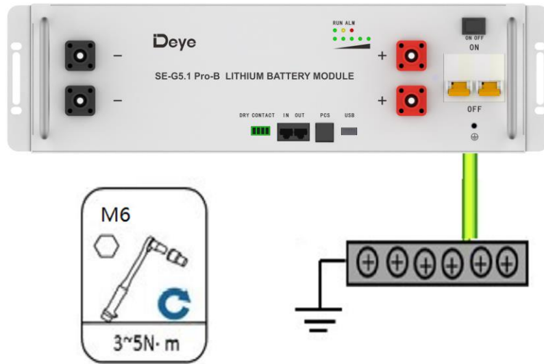
Figure 5-1: Install the Grounding Wire
