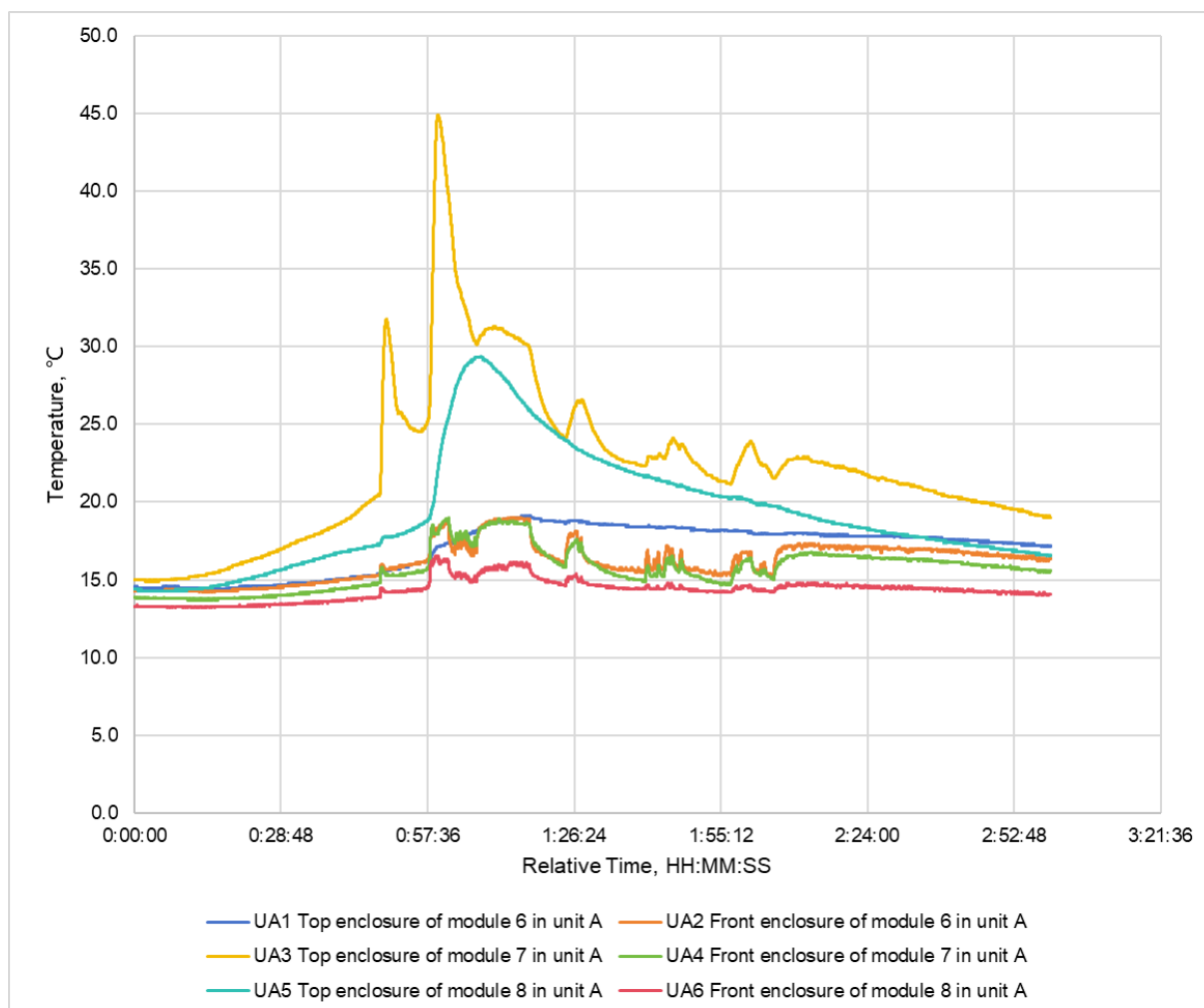
Figure 24. Temperature measurement results on the initiating unit.
